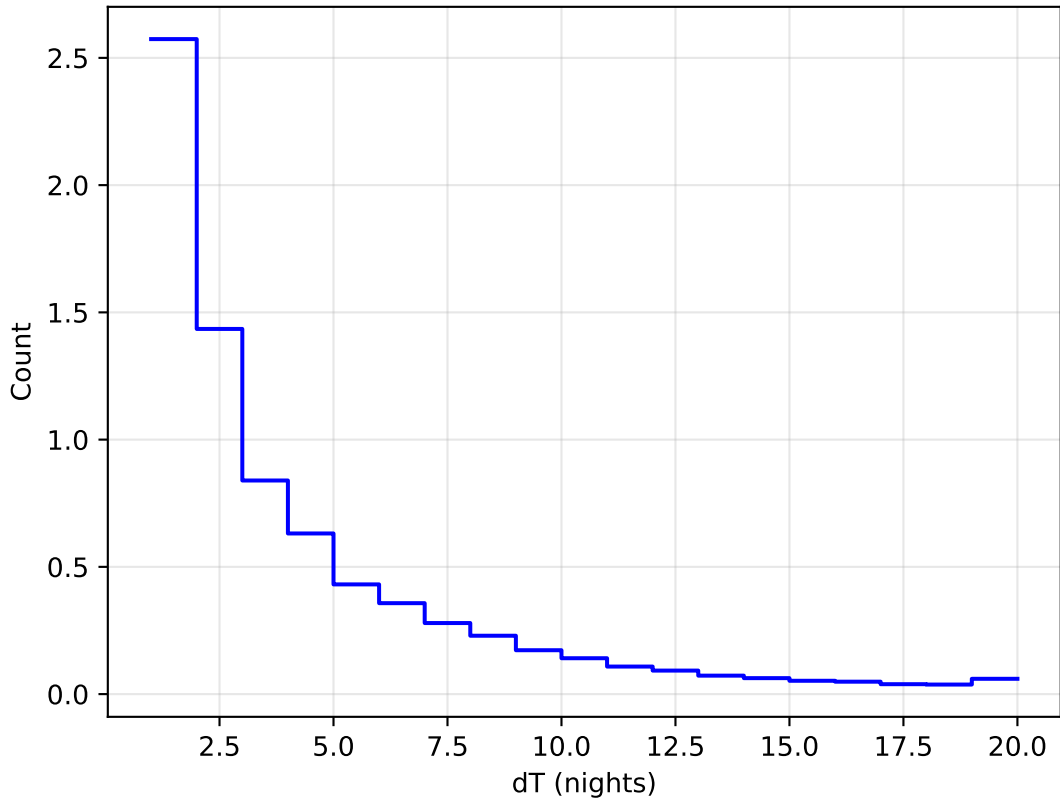
extra_ss_neo2_v3.4_10yrs WFD all bands: DeltaNight Histogram 1e6
