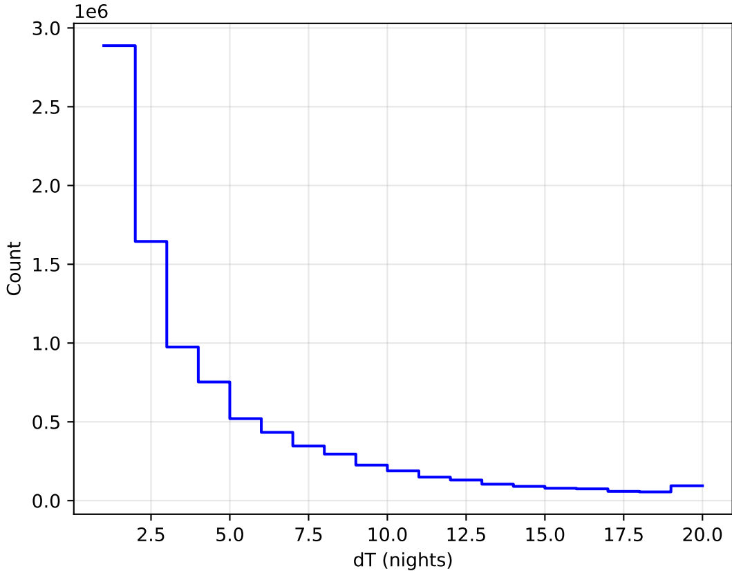
extra_ss_neo2_v3.4_10yrs All sky all bands: DeltaNight Histogram
