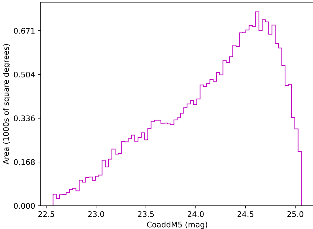
extra_ss_neo2_v3.4_10yrs Yr 3-4 z band: CoaddM5
