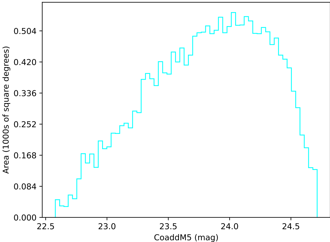
extra_ss_neo2_v3.4_10yrs Yr 3-4 u band: CoaddM5
