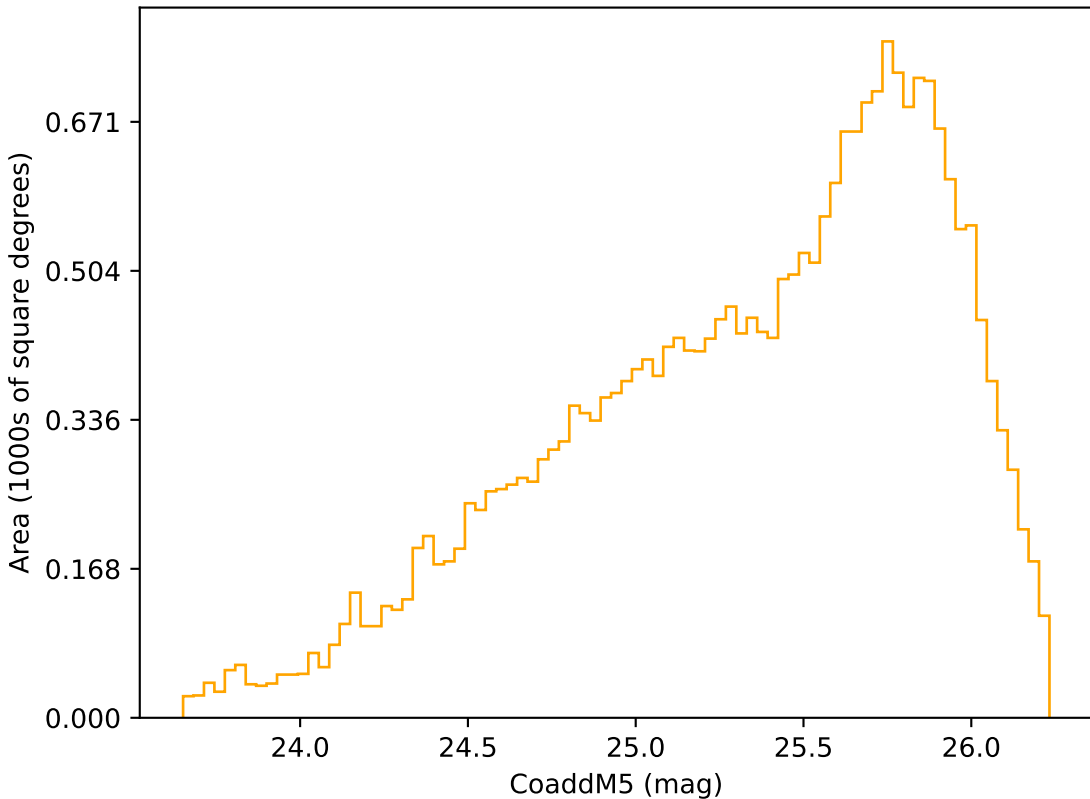
extra_ss_neo2_v3.4_10yrs Yr 3-4 r band: CoaddM5
