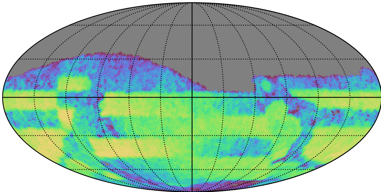
extra_ss_neo2_v3.4_10yrs Yr 3-4 i band: CoaddM5
