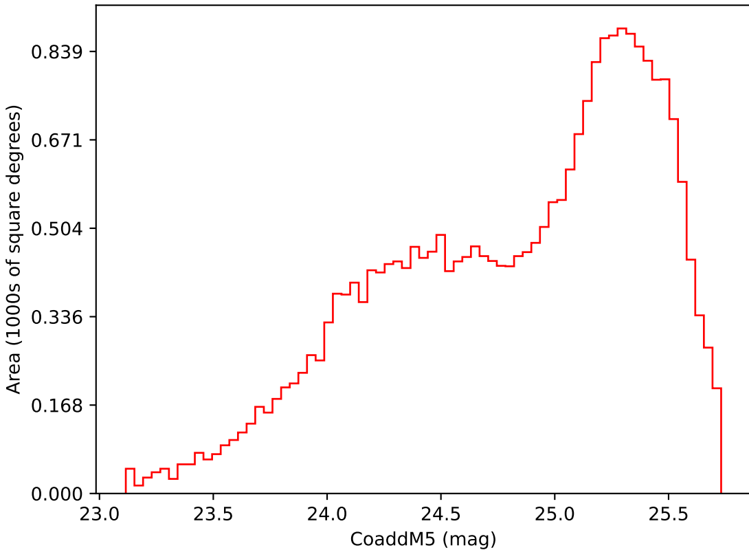
extra_ss_neo2_v3.4_10yrs Yr 3-4 i band: CoaddM5
