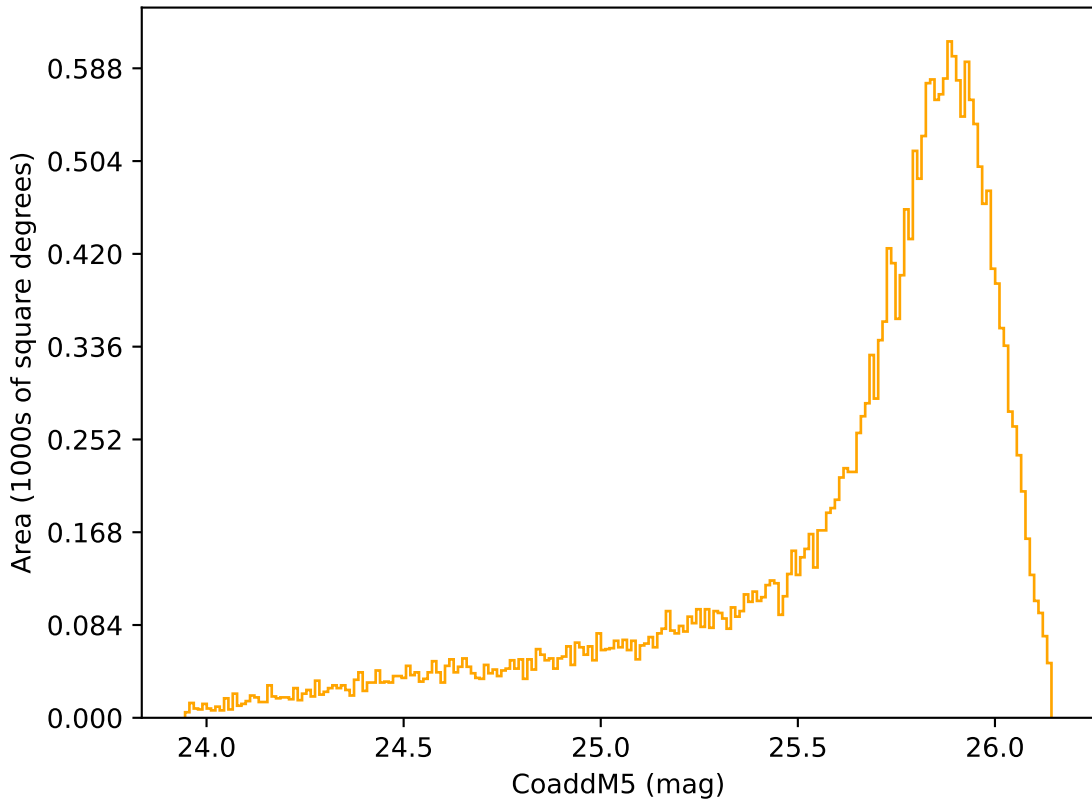
extra_ss_neo2_v3.4_10yrs Yr 1 r band: CoaddM5
