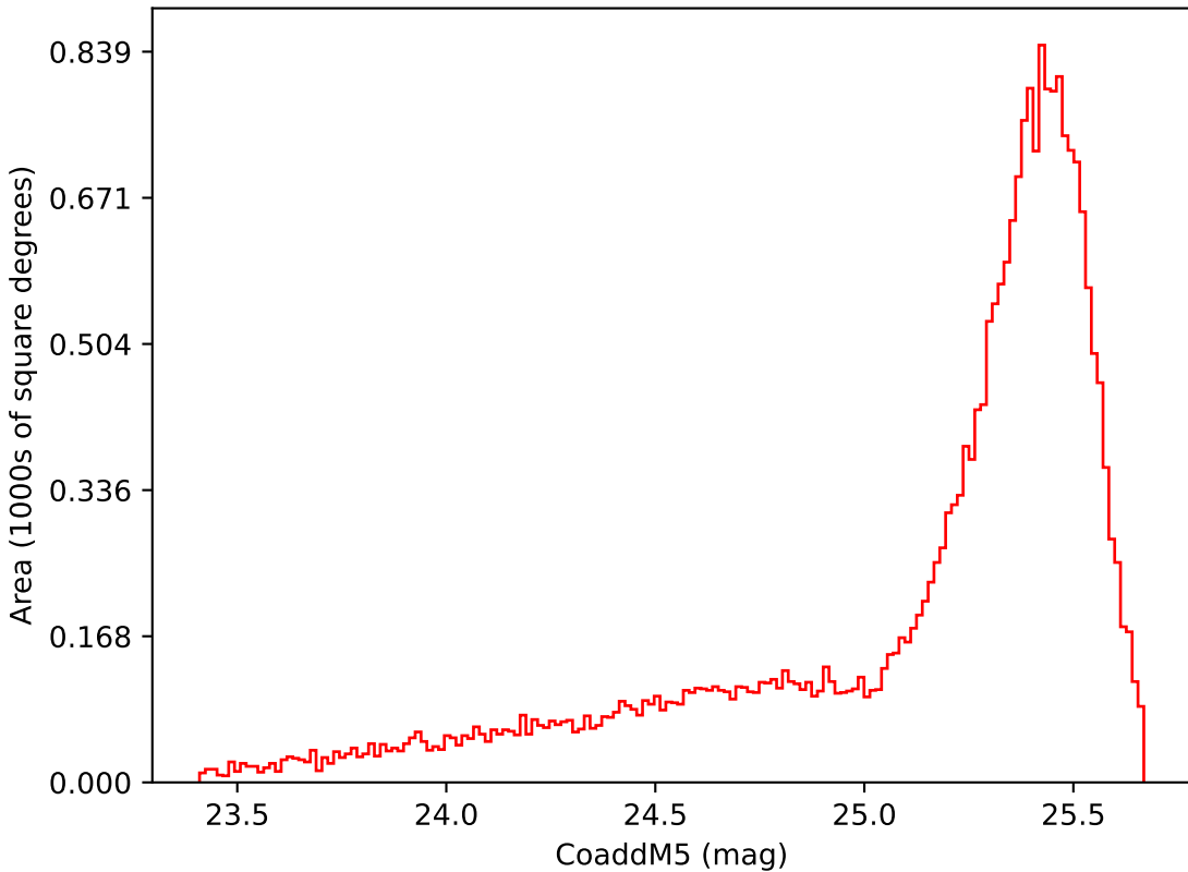
extra_ss_neo2_v3.4_10yrs Yr 1 i band: CoaddM5
