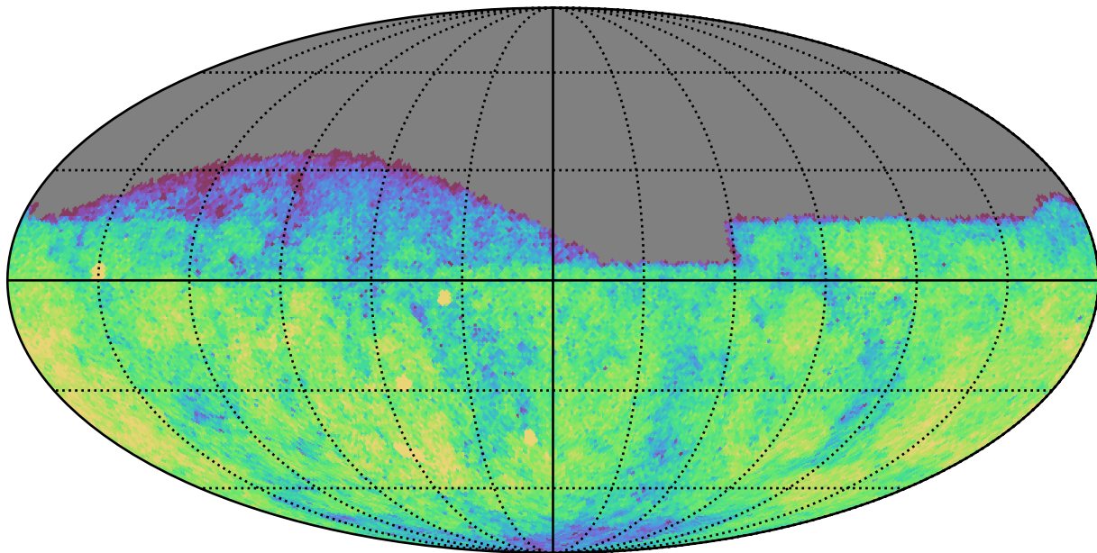
extra_ss_neo2_v3.4_10yrs Yr 1 g band: CoaddM5
