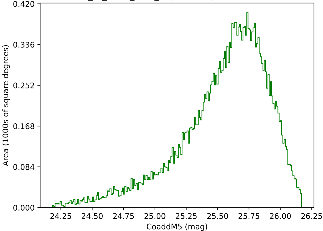
extra_ss_neo2_v3.4_10yrs Yr 1 g band: CoaddM5
