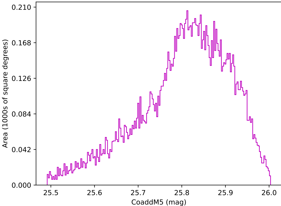
extra_ss_neo2_v3.4_10yrs WFD z band: CoaddM5
