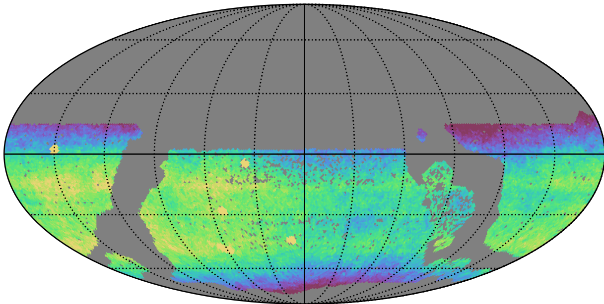
extra_ss_neo2_v3.4_10yrs WFD i band: CoaddM5
