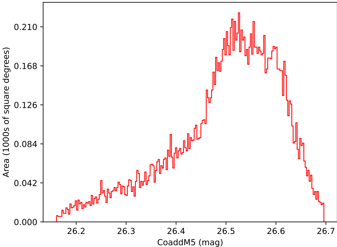
extra_ss_neo2_v3.4_10yrs WFD i band: CoaddM5
