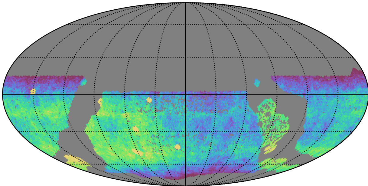
extra_ss_neo2_v3.4_10yrs WFD g band: CoaddM5
