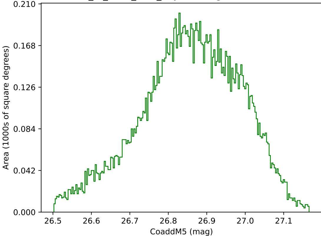
extra_ss_neo2_v3.4_10yrs WFD g band: CoaddM5
