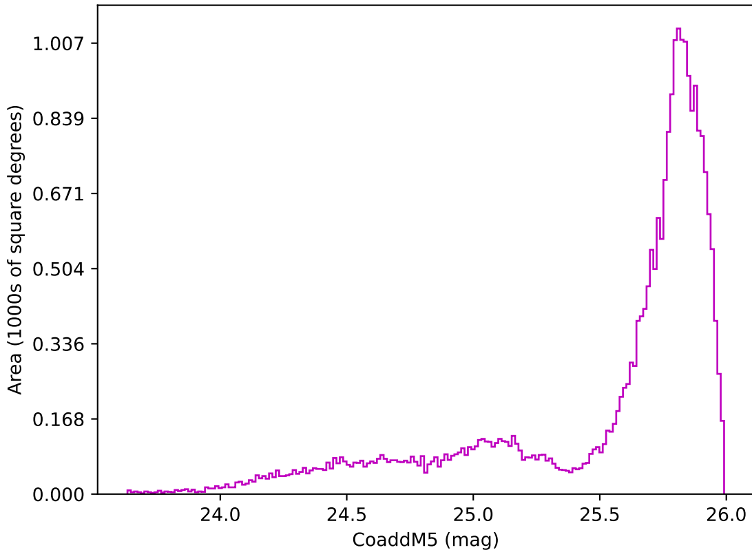
extra_ss_neo2_v3.4_10yrs All sky z band: CoaddM5
