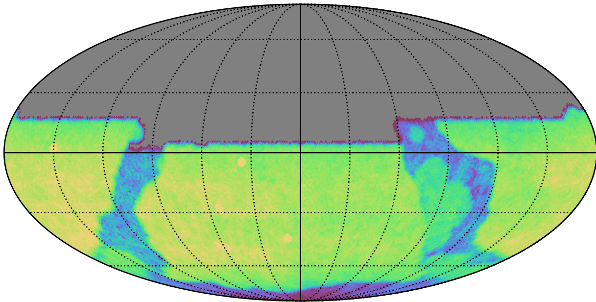
extra_ss_neo2_v3.4_10yrs All sky u band: CoaddM5
