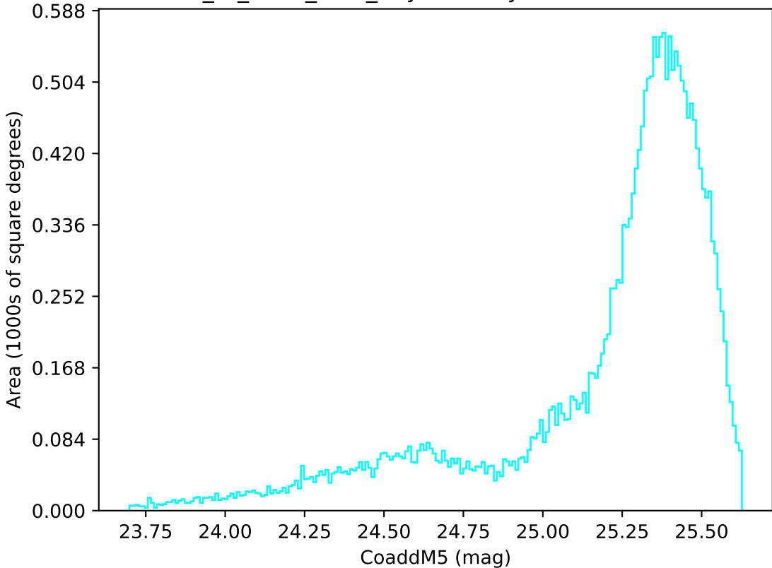
extra_ss_neo2_v3.4_10yrs All sky u band: CoaddM5
