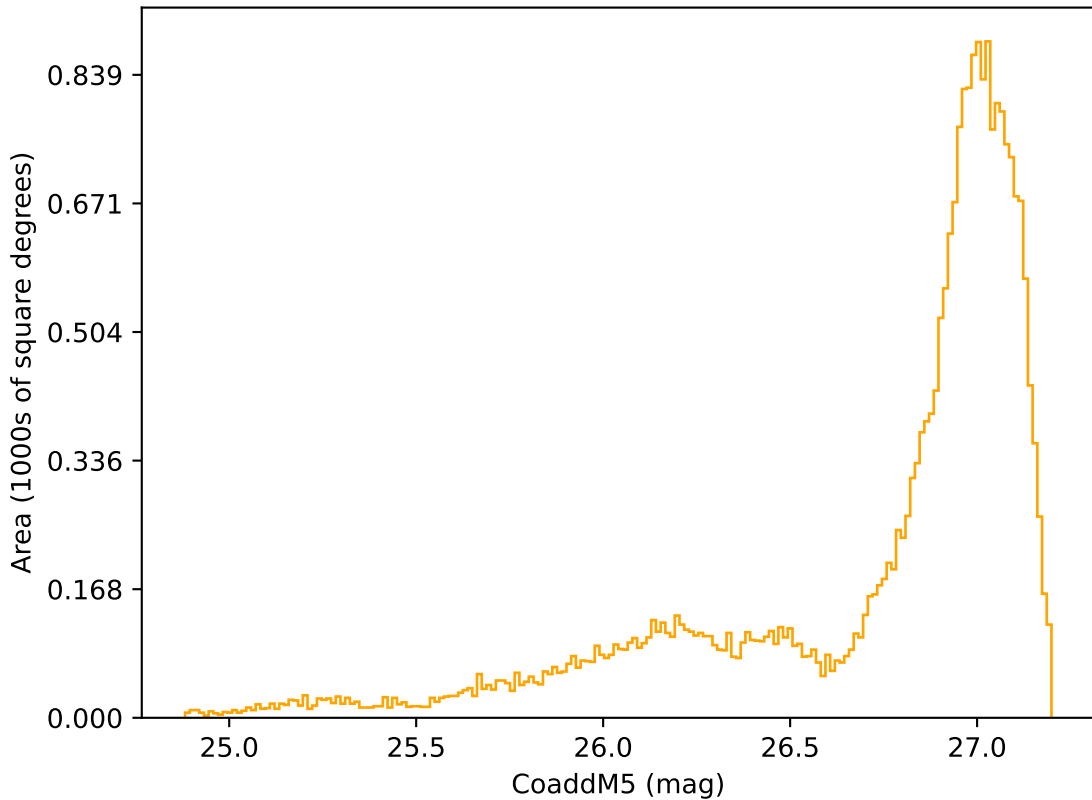
extra_ss_neo2_v3.4_10yrs All sky r band: CoaddM5
