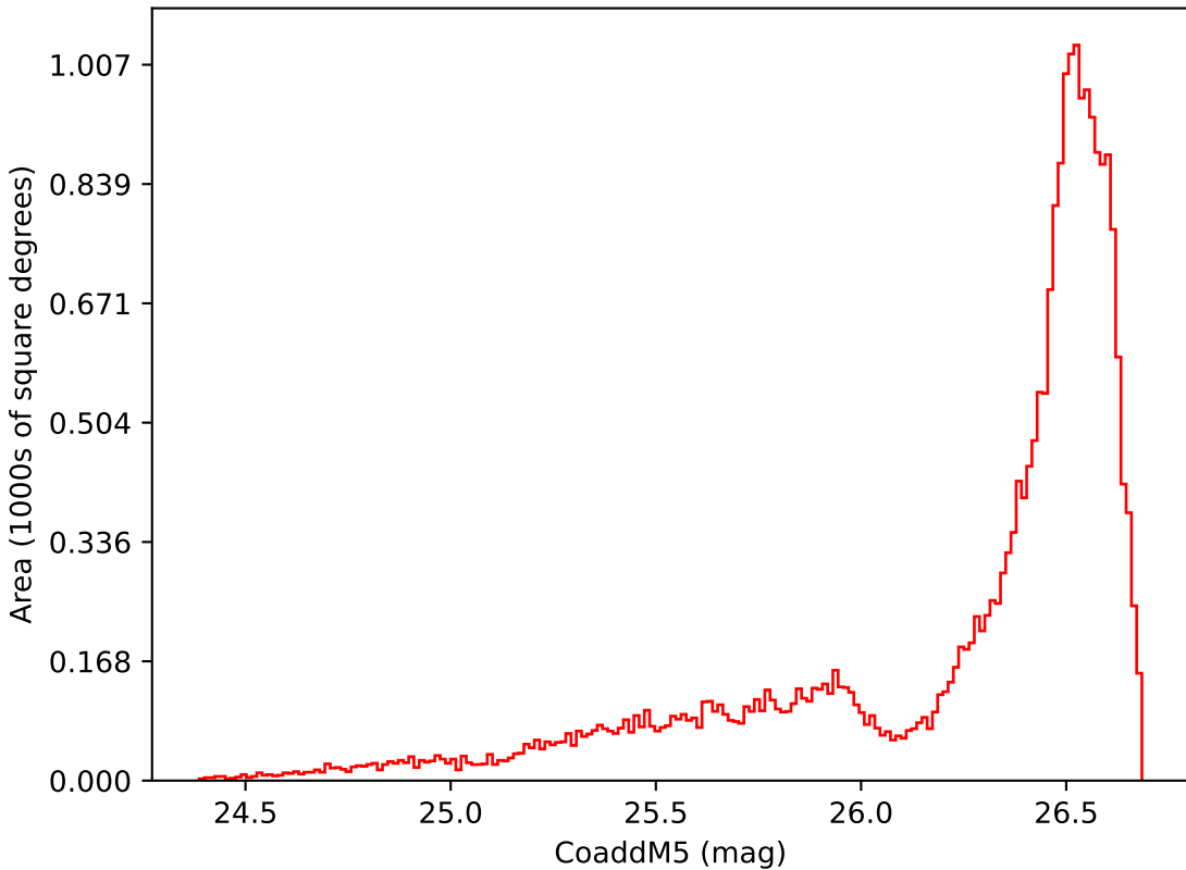
extra_ss_neo2_v3.4_10yrs All sky i band: CoaddM5
