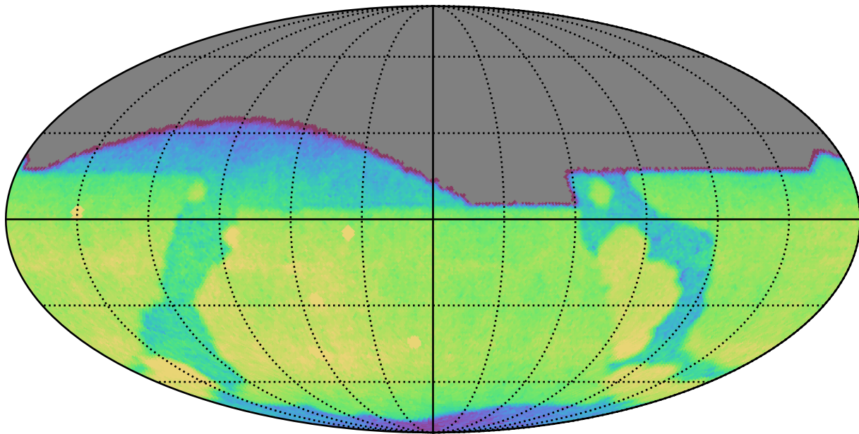
extra_ss_neo2_v3.4_10yrs All sky g band: CoaddM5
