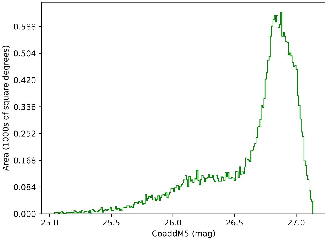
extra_ss_neo2_v3.4_10yrs All sky g band: CoaddM5
