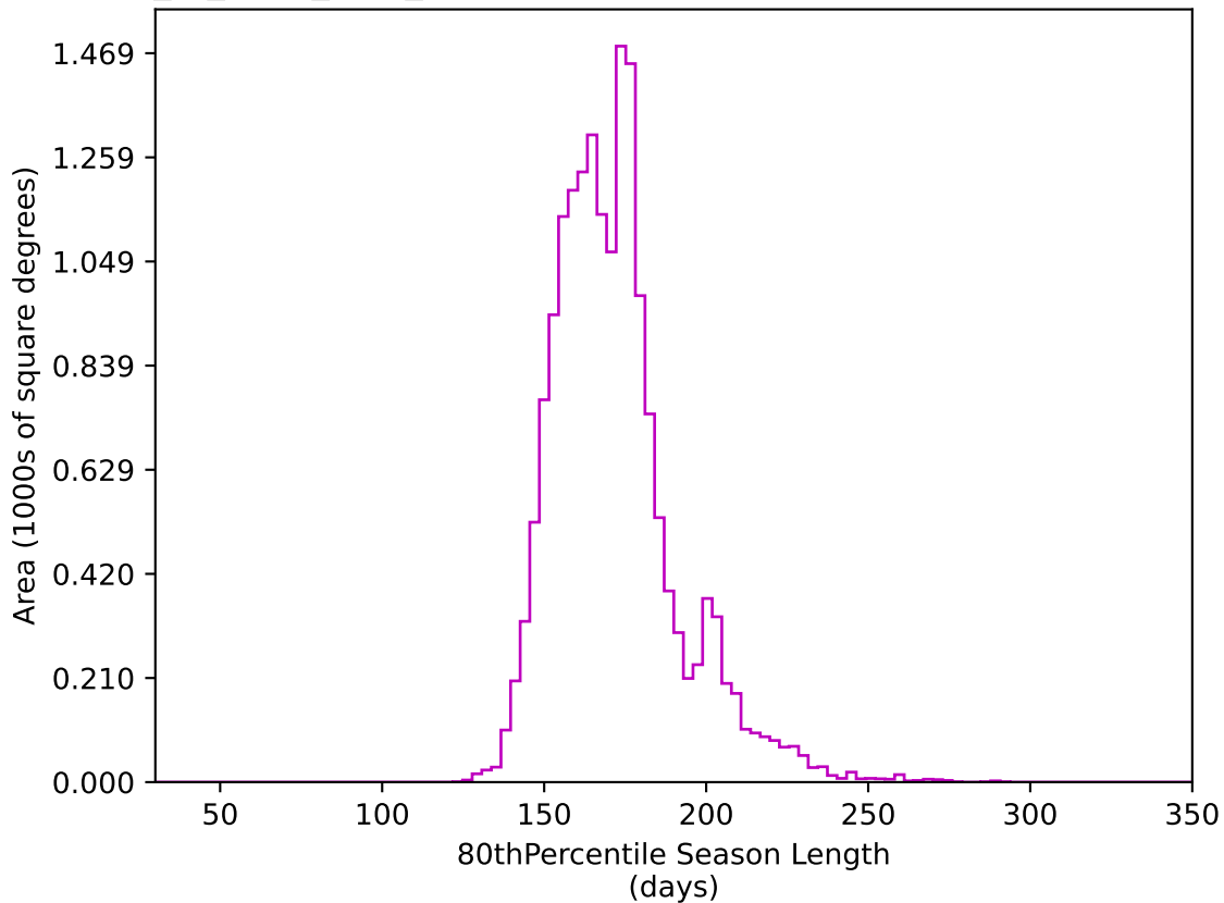
extra_ss_neo2_v3.4_10yrs WFD z band: 80thPercentile Season Length
