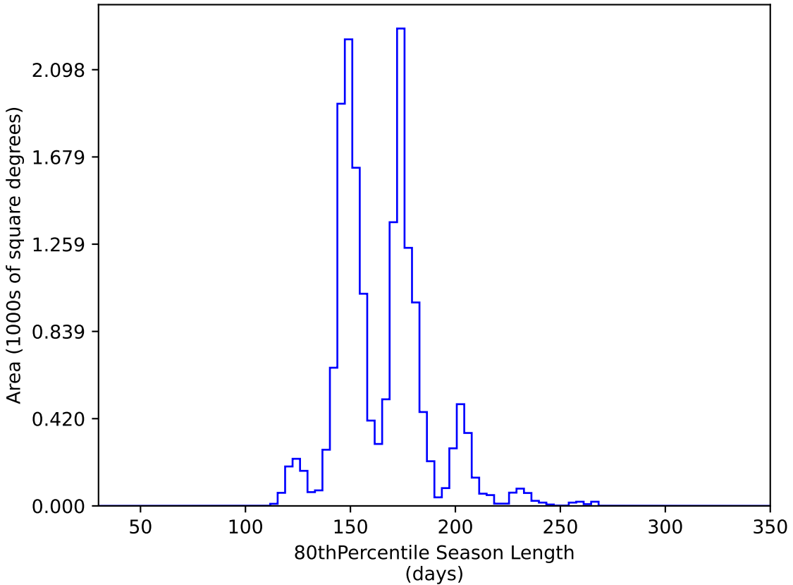
extra_ss_neo2_v3.4_10yrs WFD y band: 80thPercentile Season Length
