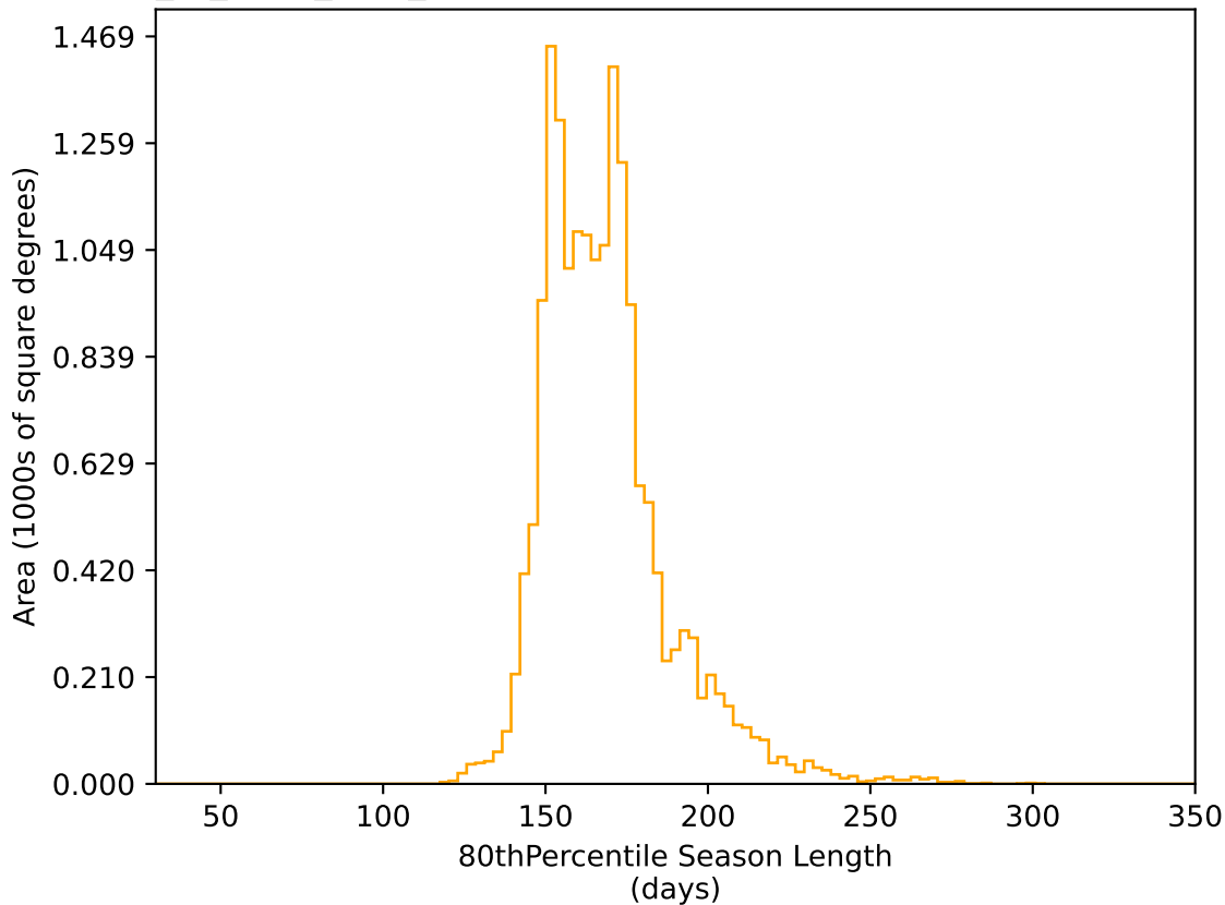
extra_ss_neo2_v3.4_10yrs WFD r band: 80thPercentile Season Length
