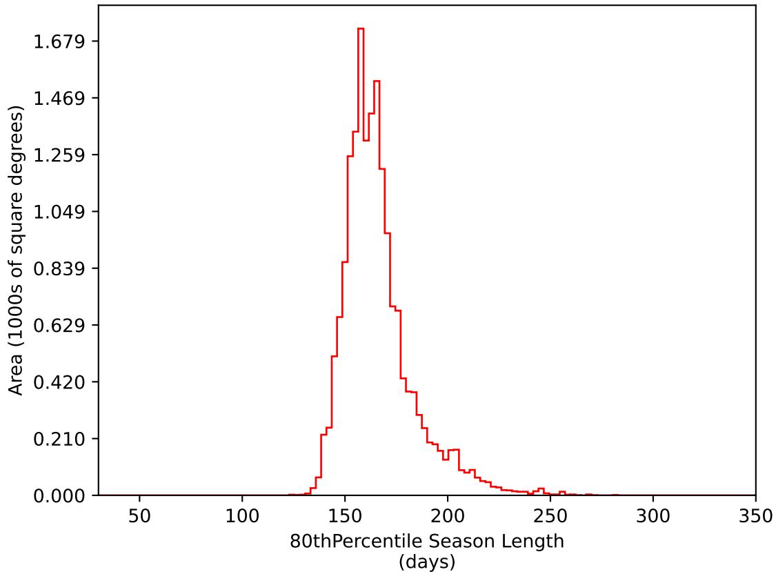
extra_ss_neo2_v3.4_10yrs WFD i band: 80thPercentile Season Length
