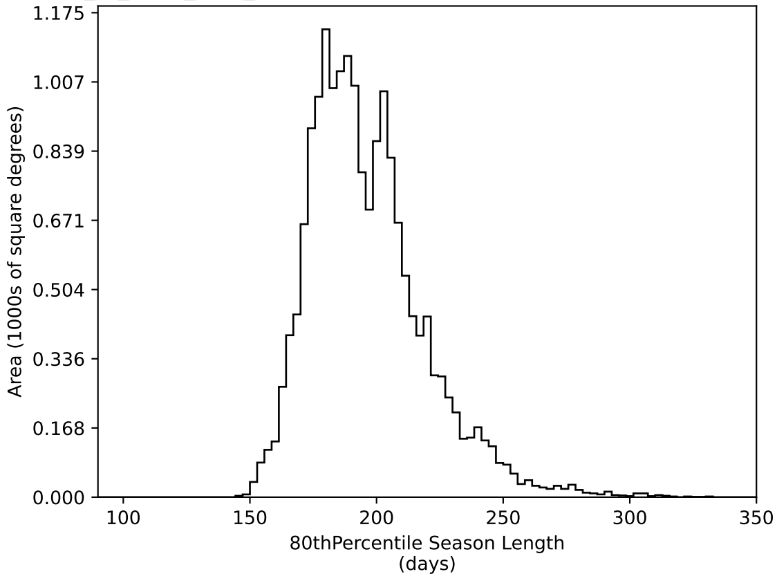
extra_ss_neo2_v3.4_10yrs WFD all bands: 80thPercentile Season Length
