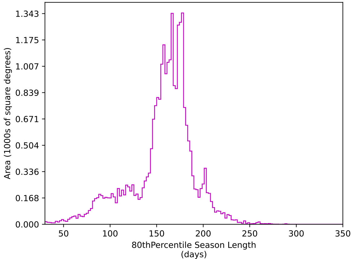
extra_ss_neo2_v3.4_10yrs All sky z band: 80thPercentile Season Length
