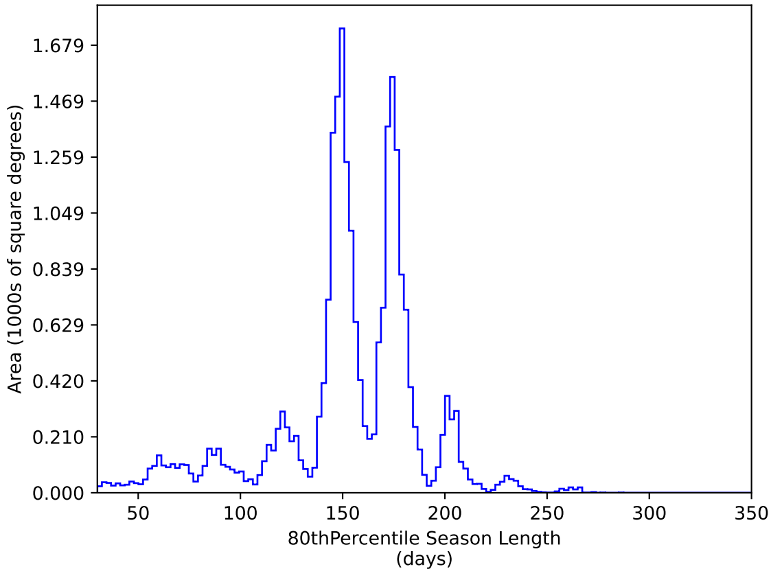
extra_ss_neo2_v3.4_10yrs All sky y band: 80thPercentile Season Length
