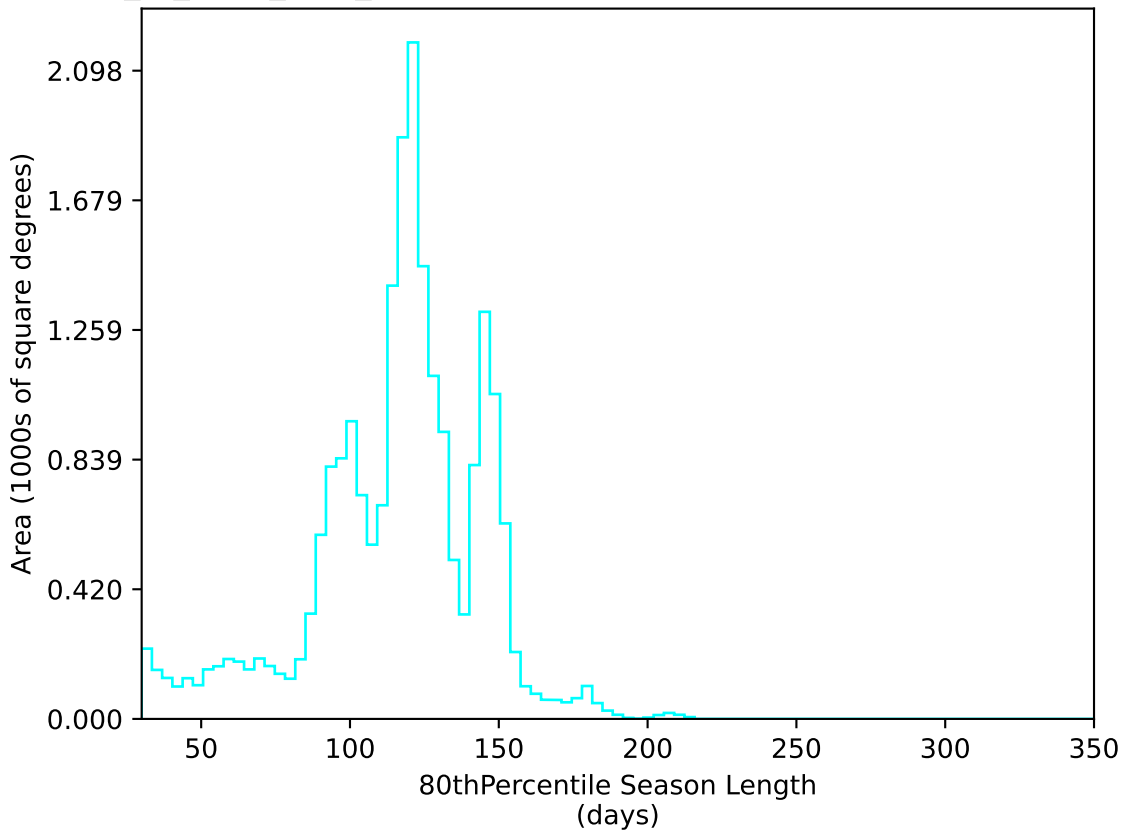
extra_ss_neo2_v3.4_10yrs All sky u band: 80thPercentile Season Length
