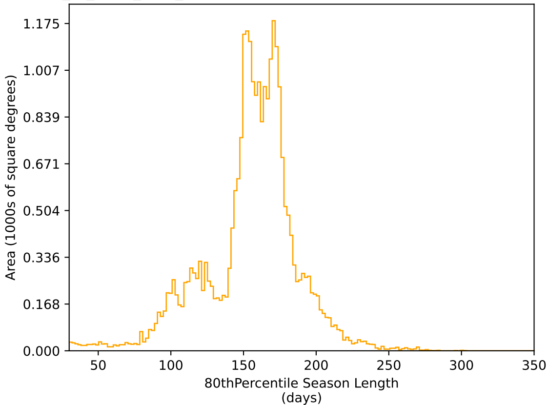
extra_ss_neo2_v3.4_10yrs All sky r band: 80thPercentile Season Length
