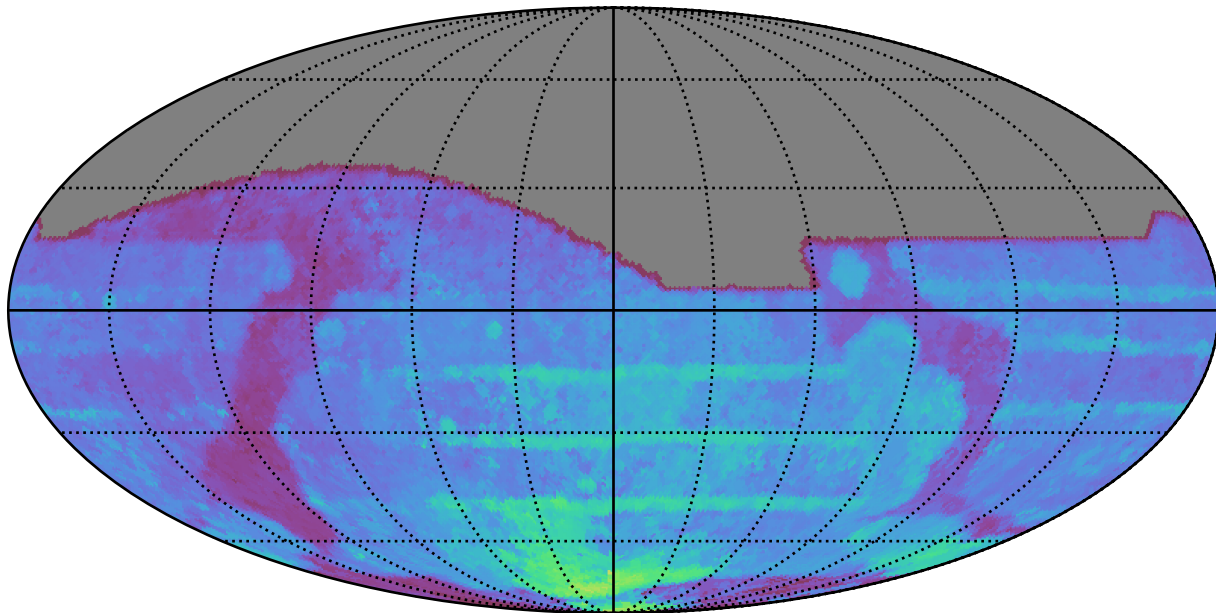
extra_ss_neo2_v3.4_10yrs All sky all bands: 80thPercentile Season Length
