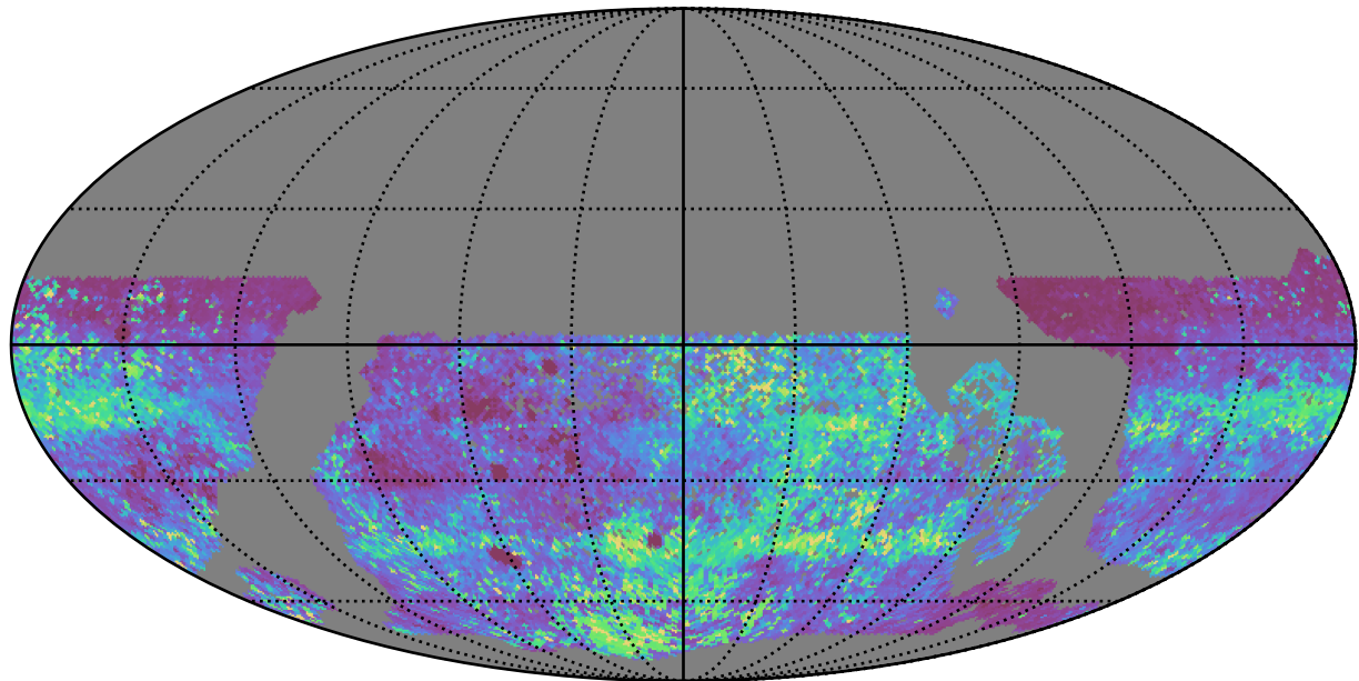
extra_ss_neo2_v3.4_10yrs WFD zy bands: 75th Percentile Intranight Timespan
