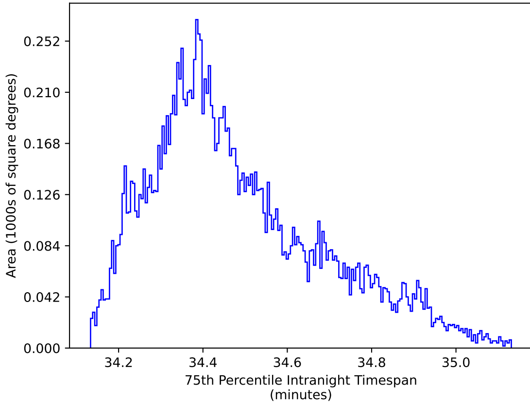
extra_ss_neo2_v3.4_10yrs WFD zy bands: 75th Percentile Intranight Timespan
