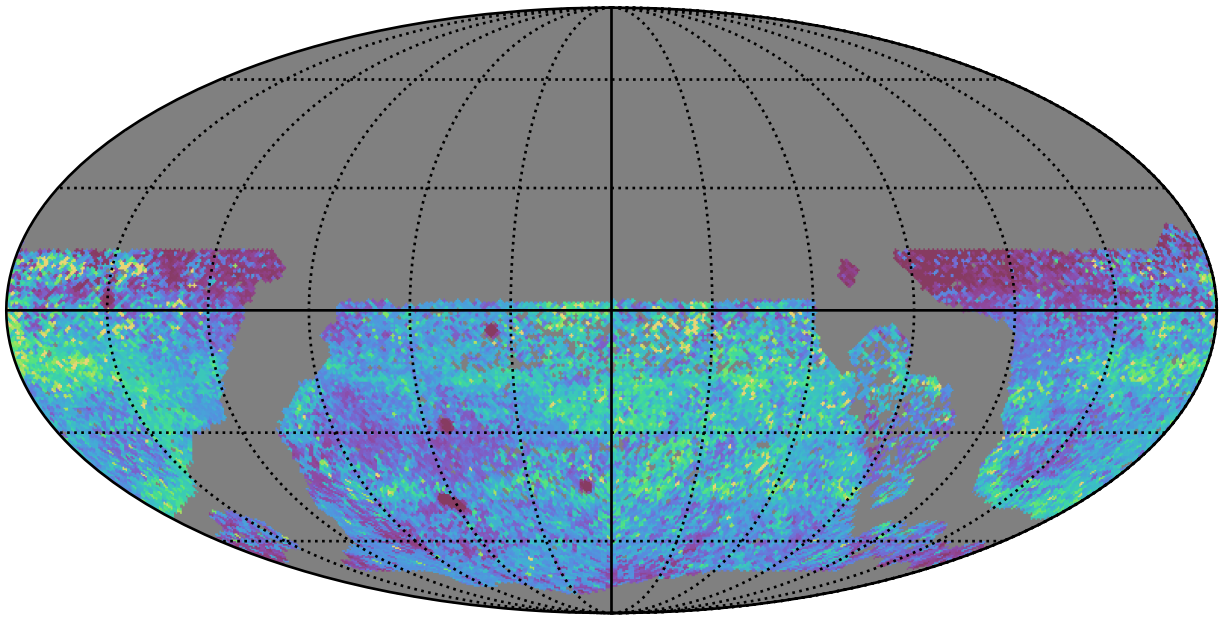
extra_ss_neo2_v3.4_10yrs WFD y band: 75th Percentile Intranight Timespan
