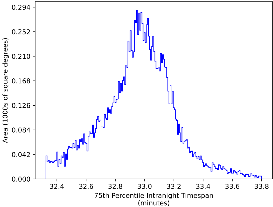
extra_ss_neo2_v3.4_10yrs WFD y band: 75th Percentile Intranight Timespan
