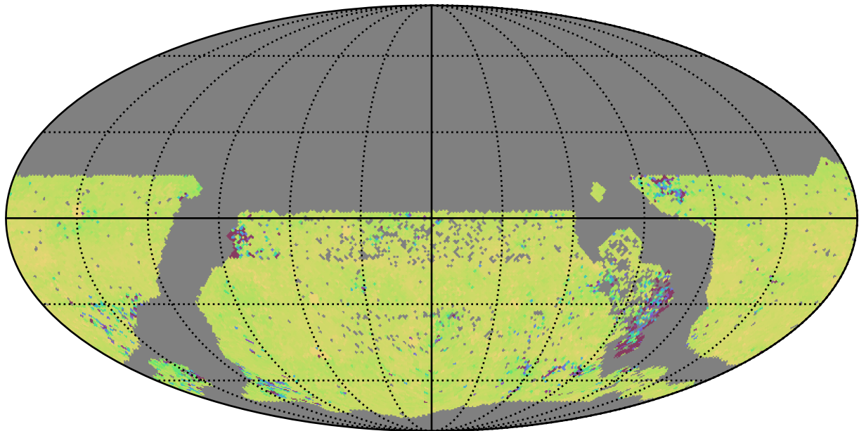
extra_ss_neo2_v3.4_10yrs WFD ug bands: 75th Percentile Intranight Timespan
