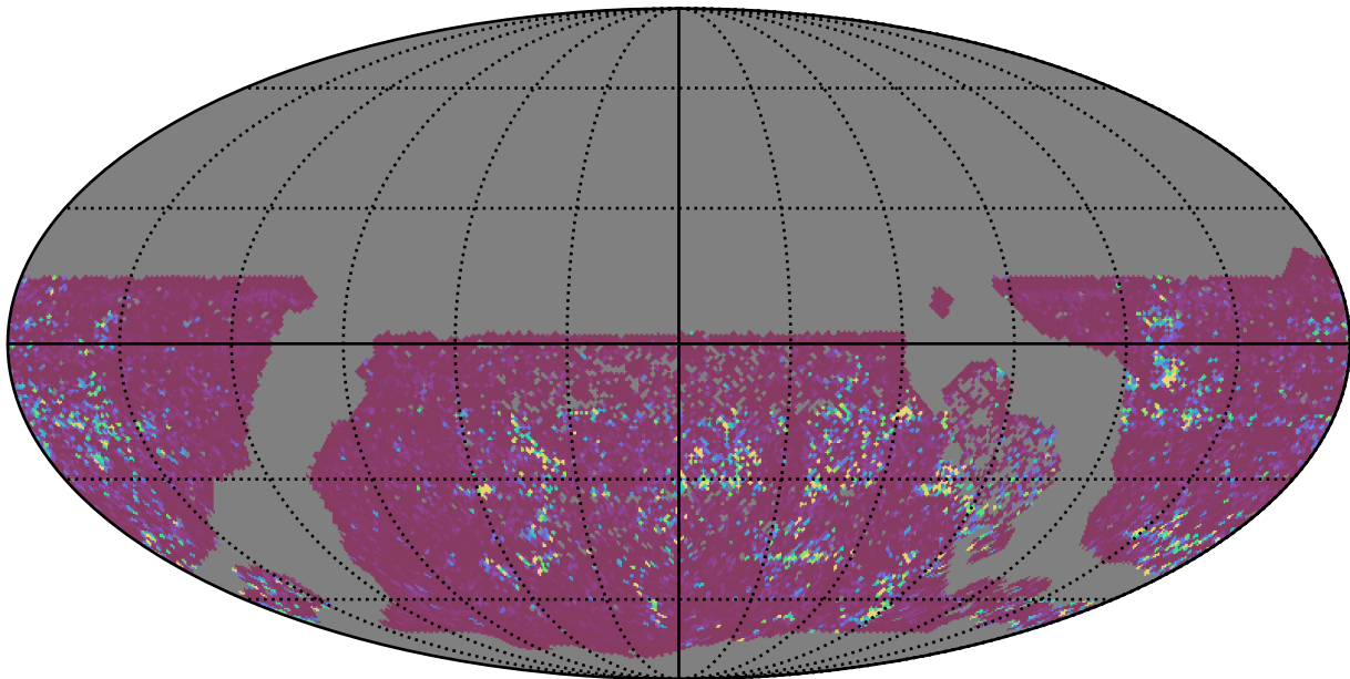
extra_ss_neo2_v3.4_10yrs WFD u band: 75th Percentile Intranight Timespan
