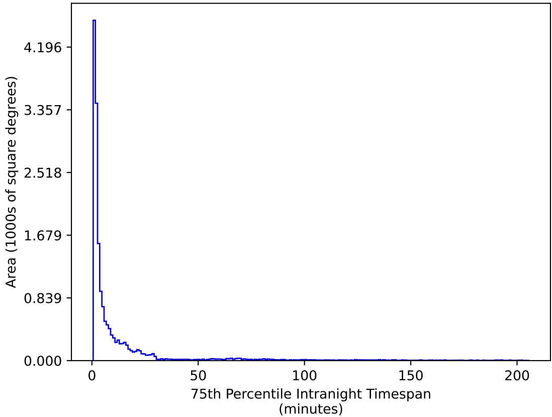
extra_ss_neo2_v3.4_10yrs WFD u band: 75th Percentile Intranight Timespan
