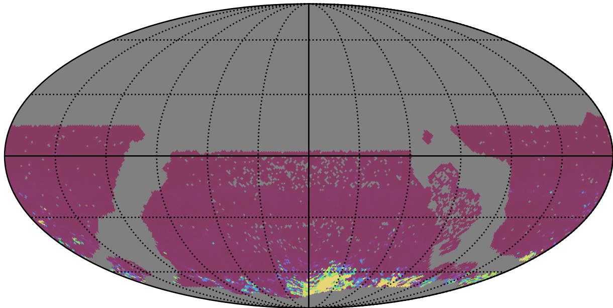
extra_ss_neo2_v3.4_10yrs WFD ri bands: 75th Percentile Intranight Timespan
