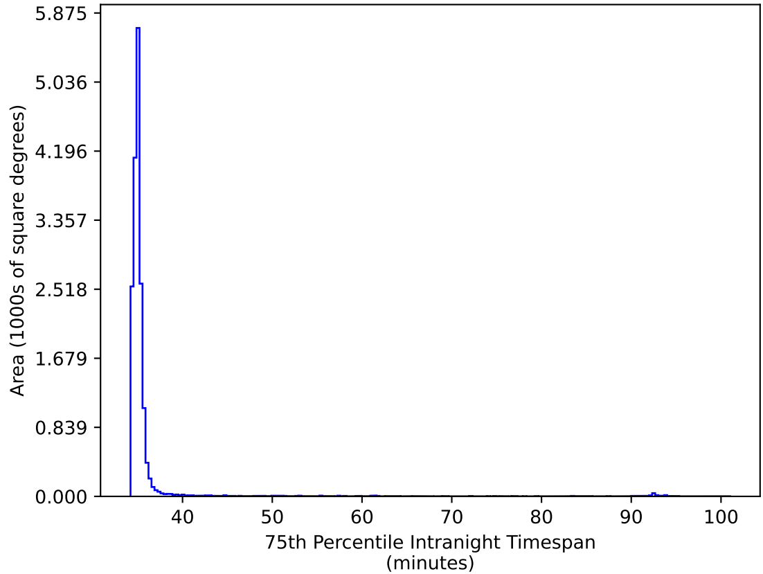
extra_ss_neo2_v3.4_10yrs WFD ri bands: 75th Percentile Intranight Timespan
