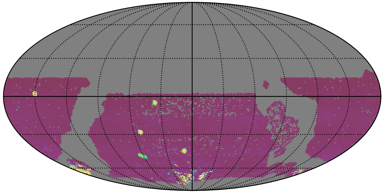
extra_ss_neo2_v3.4_10yrs WFD iz bands: 75th Percentile Intranight Timespan
