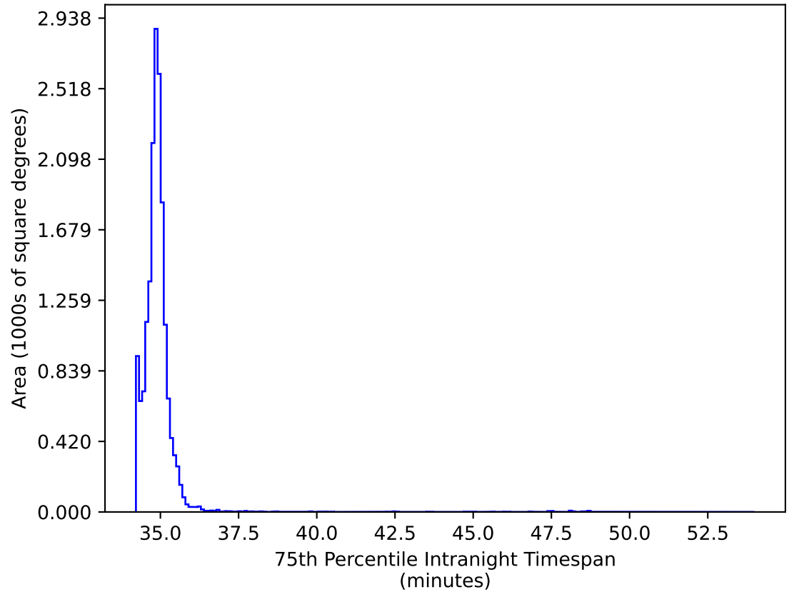
extra_ss_neo2_v3.4_10yrs WFD iz bands: 75th Percentile Intranight Timespan
