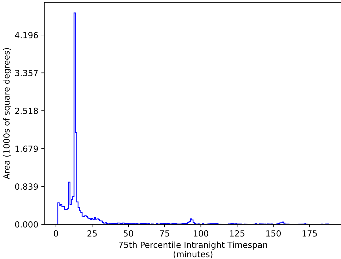
extra_ss_neo2_v3.4_10yrs WFD i band: 75th Percentile Intranight Timespan
