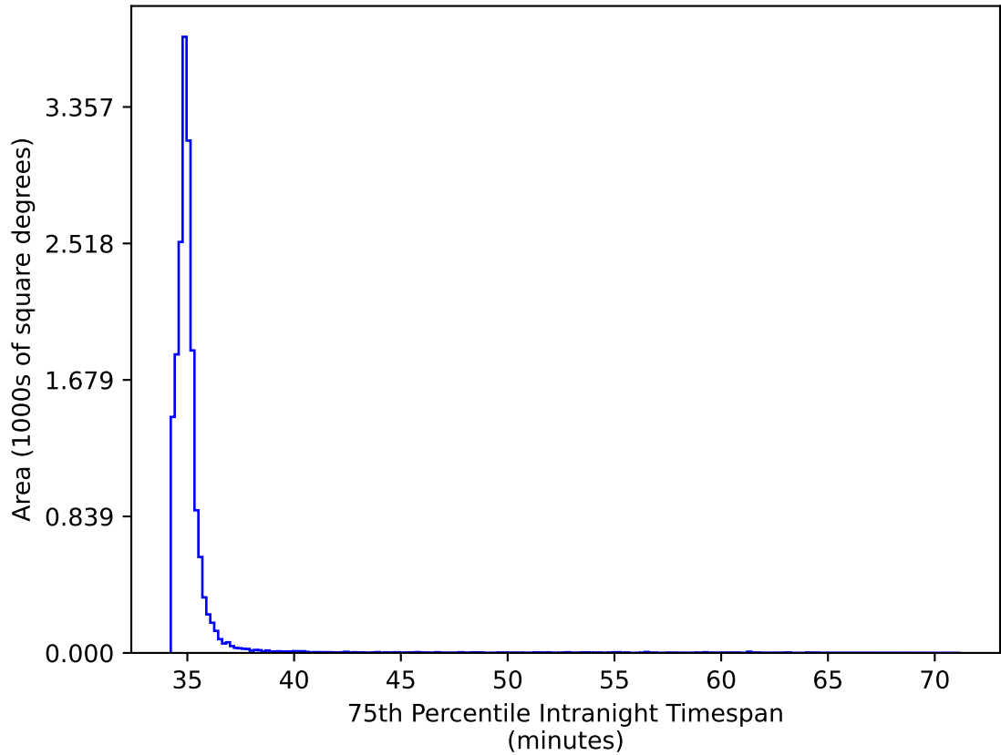
extra_ss_neo2_v3.4_10yrs WFD gr bands: 75th Percentile Intranight Timespan
