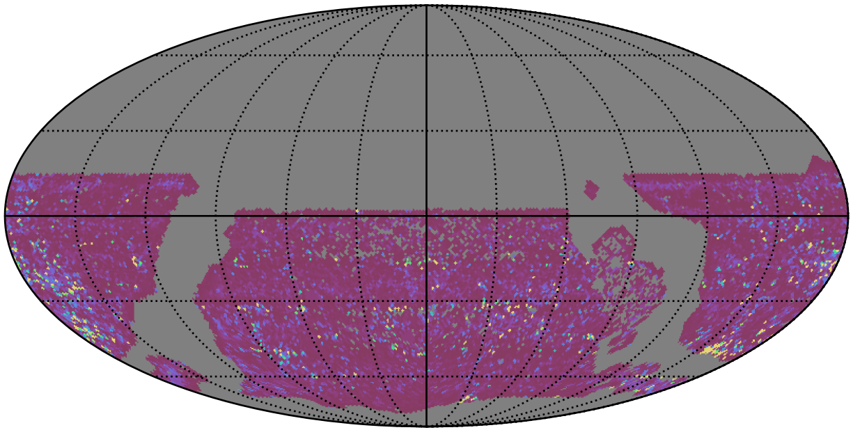
extra_ss_neo2_v3.4_10yrs WFD g band: 75th Percentile Intranight Timespan
