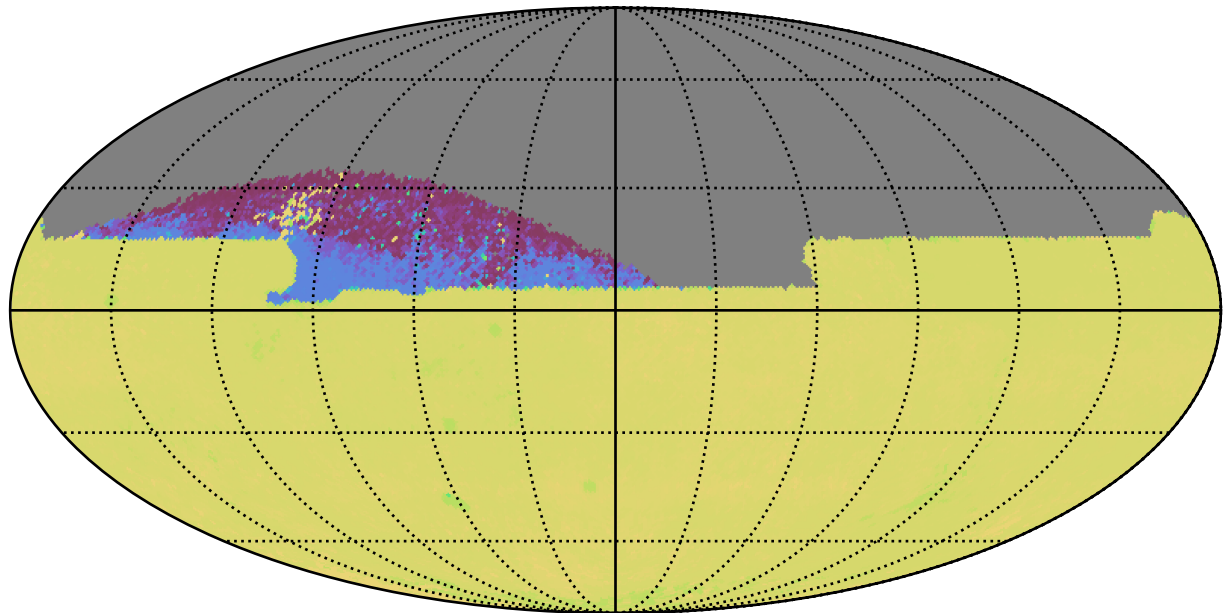
extra_ss_neo2_v3.4_10yrs All sky zy bands: 75th Percentile Intranight Timespan
