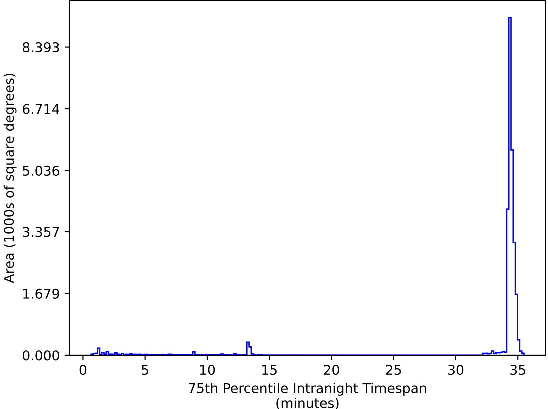
extra_ss_neo2_v3.4_10yrs All sky zy bands: 75th Percentile Intranight Timespan
