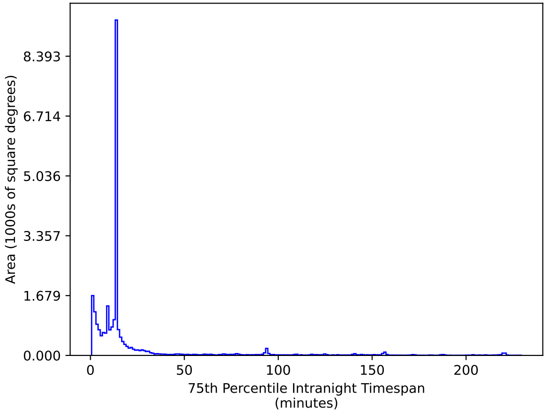
extra_ss_neo2_v3.4_10yrs All sky z band: 75th Percentile Intranight Timespan
